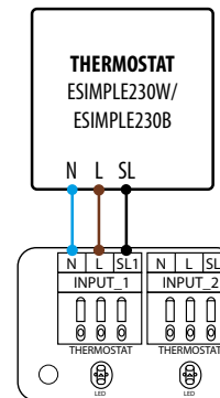
Control box ECB08M230
